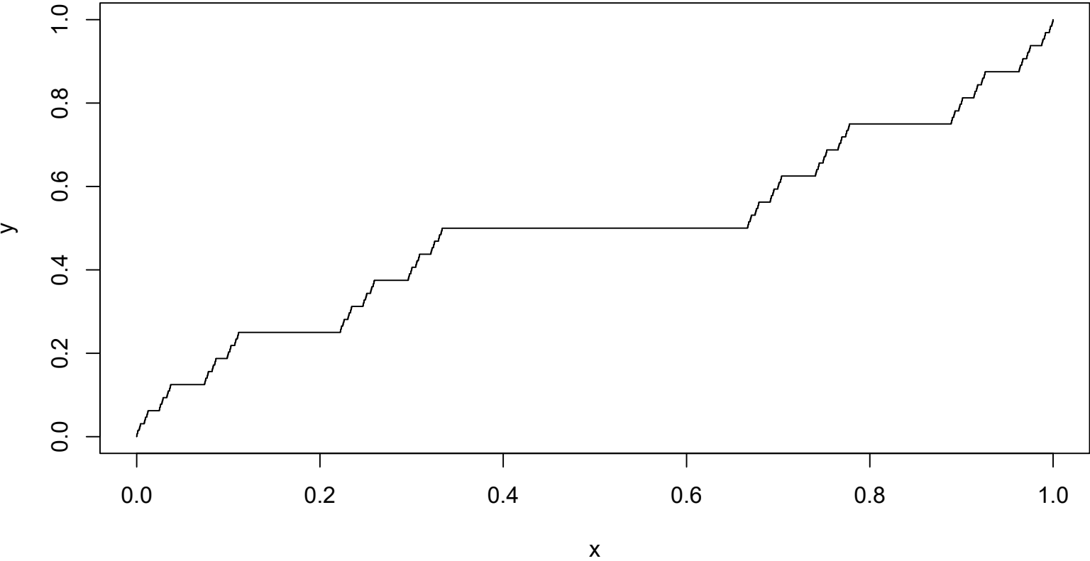
CDF which is continuous but NOT absolutely continuous
