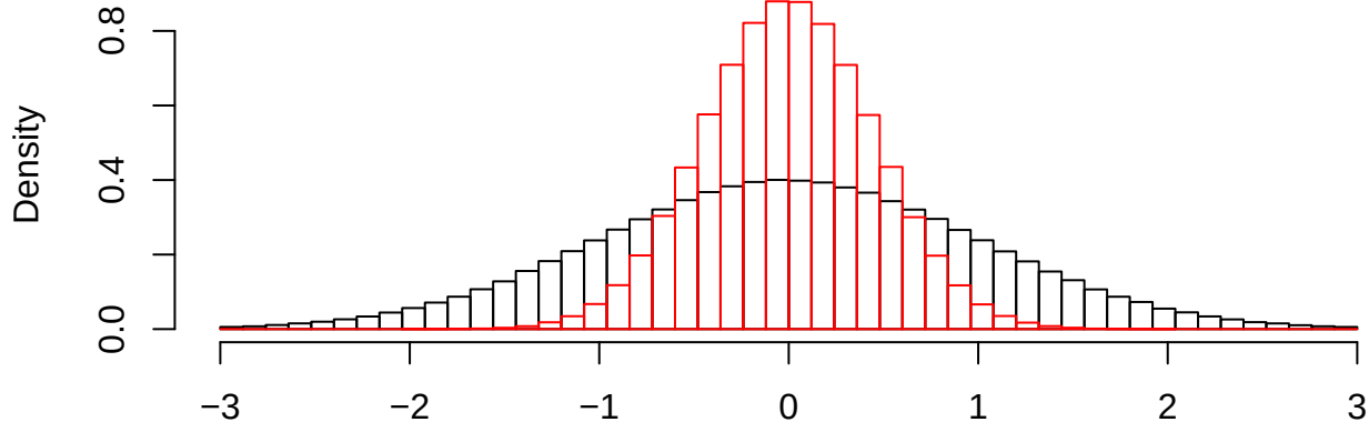
Histogram of X and Xbar for Normal Population
