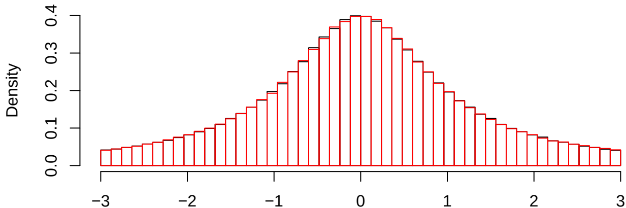
Histogram of X and Xbar for Cauchy Population
