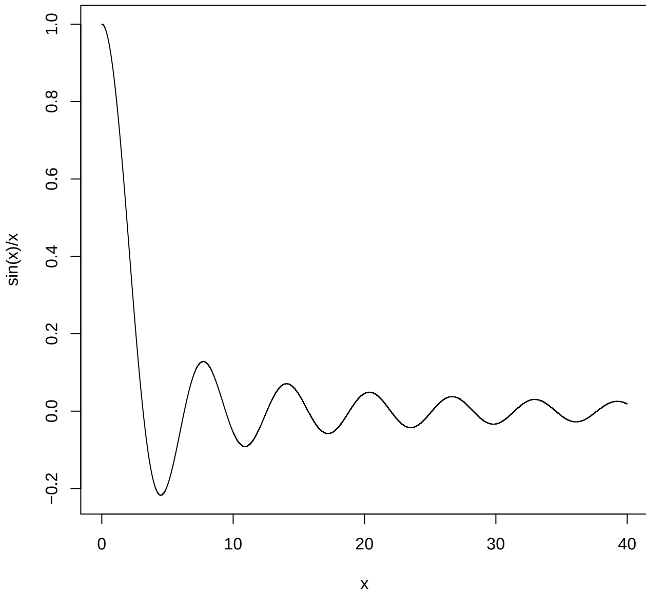
Plot of \text{Sin}(x)/x
