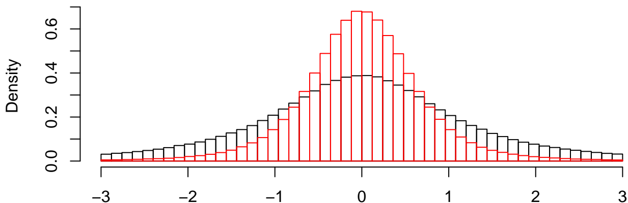
Histogram of X and Xbar for t-distribution with 2 df (sample size 10)
