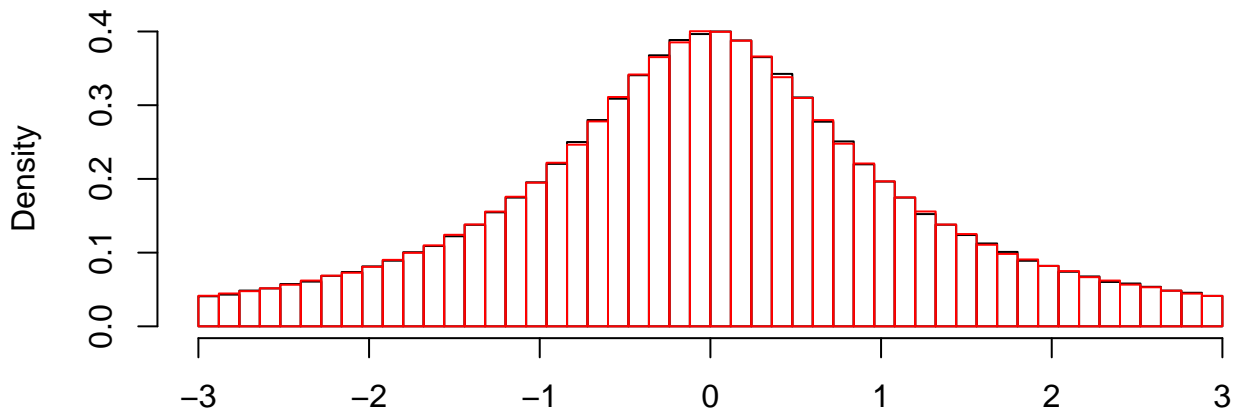
Histogram of X and Xbar for Cauchy Population (sample size 10)
