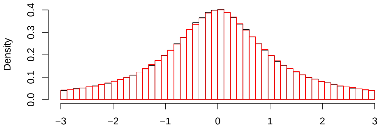
Histogram of X and Xbar for Cauchy Population (sample size 5)
