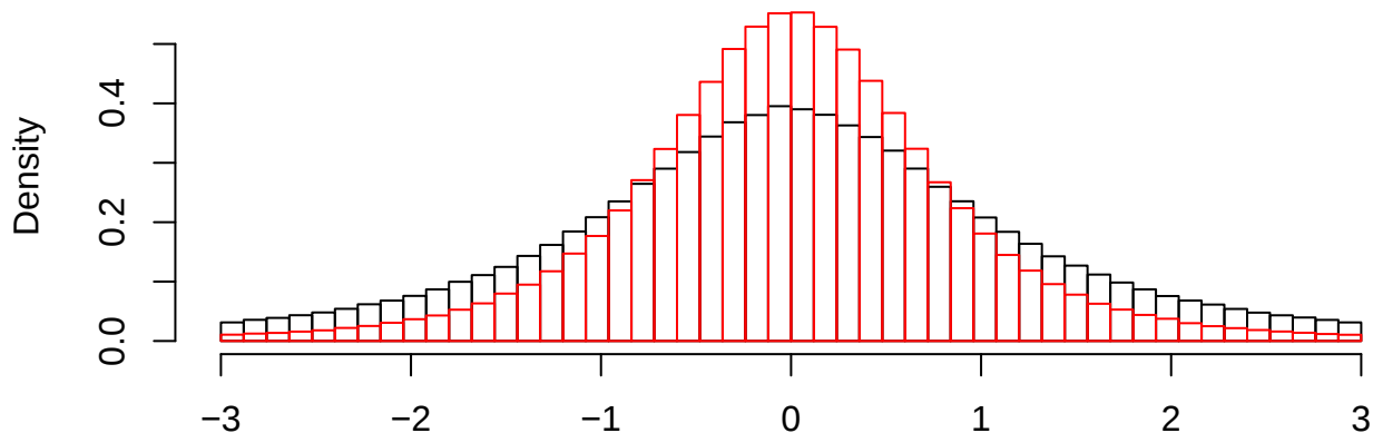
Histogram of X and Xbar for t-distribution with 2 df (sample size 5)
