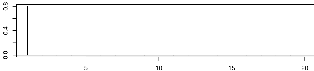
Series True PACF
