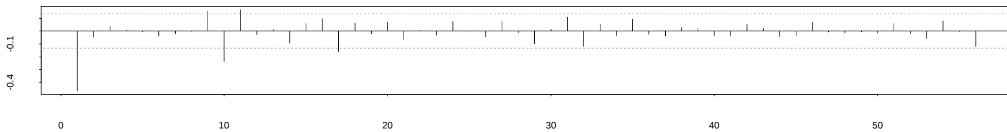
Inverse ACF
