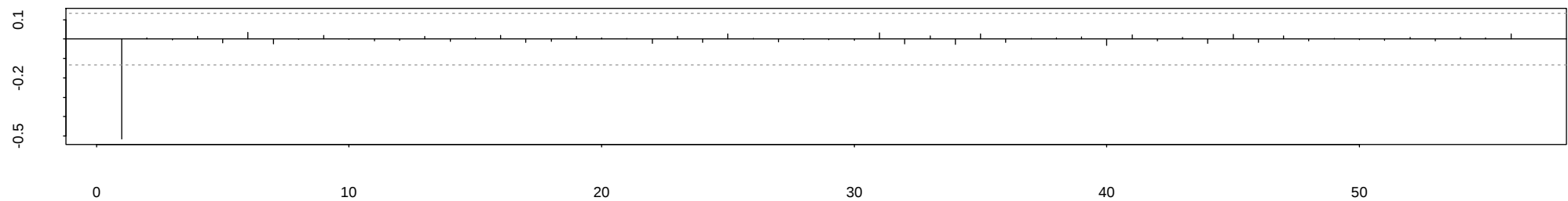
Inverse ACF
