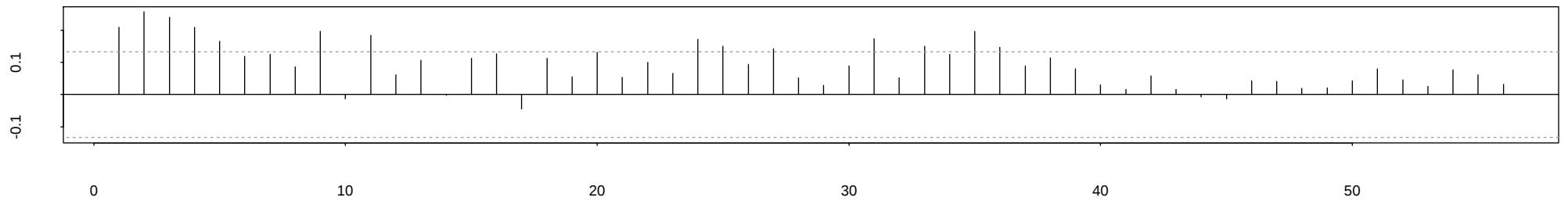
Inverse ACF
