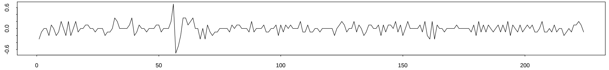
Time Series Plot : Second Differences
