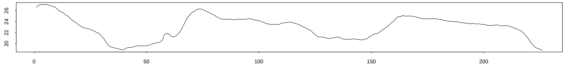
Time Series Plot : Box-Jenkins Series C
