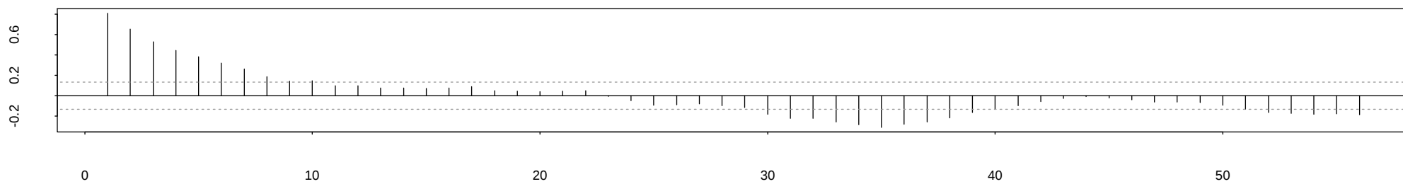
Partial ACF
