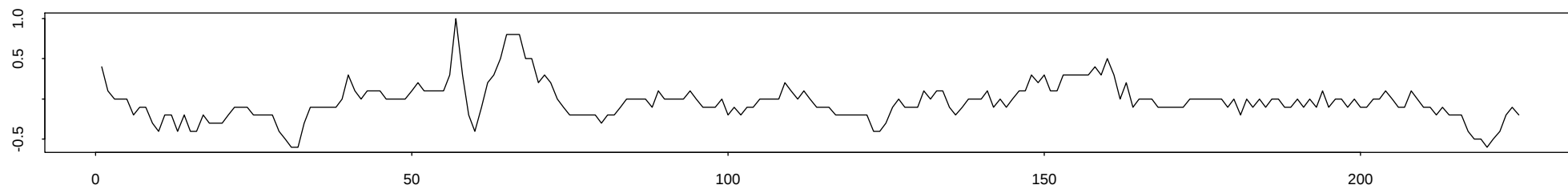
Time Series Plot : First Differences
