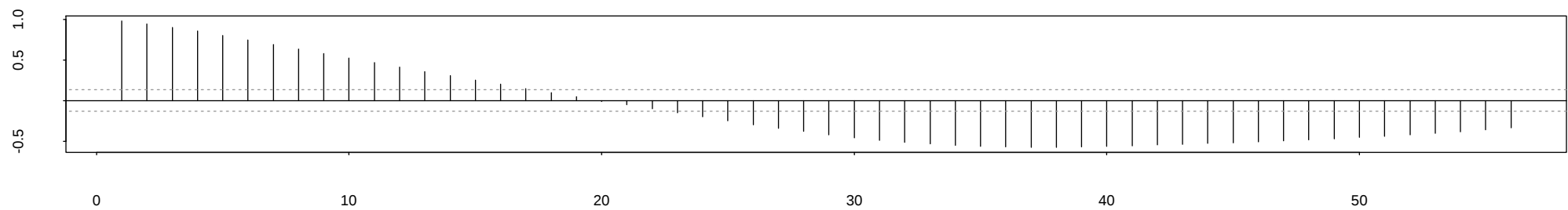
Partial ACF
