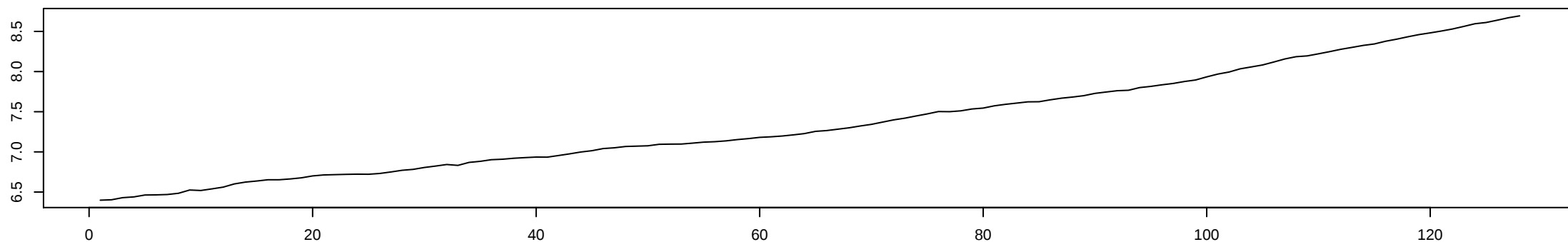
Time Series Plot: Logs of Quarterly Iowa Nonfarm Income
