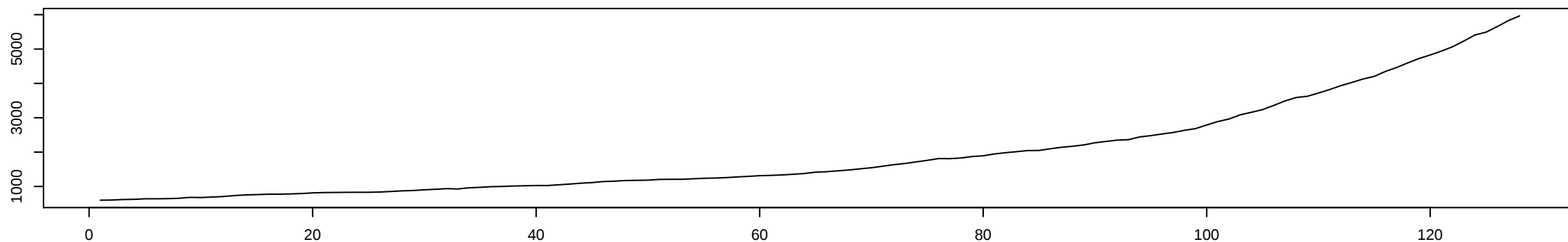
Time Series Plot: Raw Quarterly Iowa Nonfarm Income
