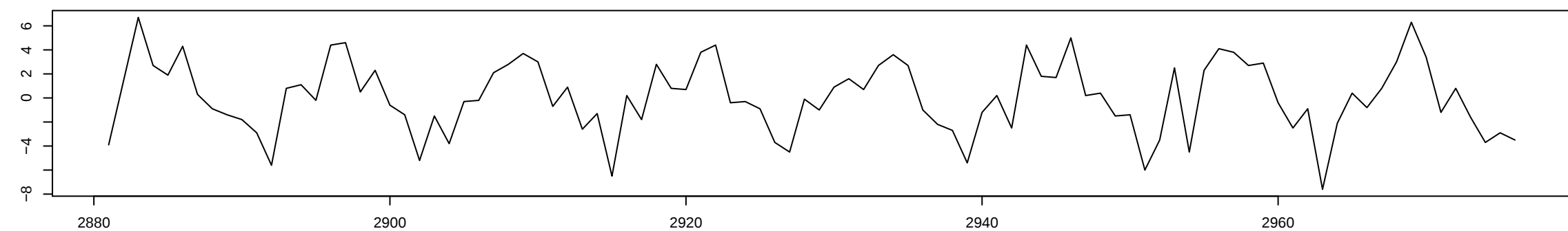
Differencing at Lag 1 -- Monthly Temperatures in England
