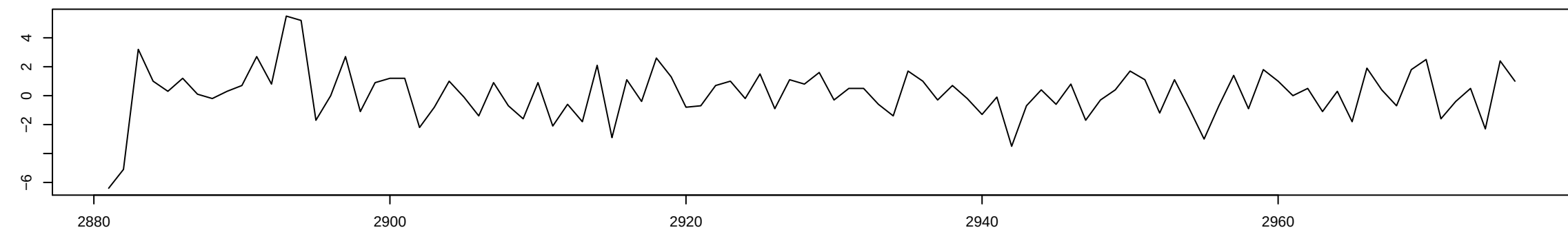
Differencing at Lag 12 -- Monthly Temperatures in England
