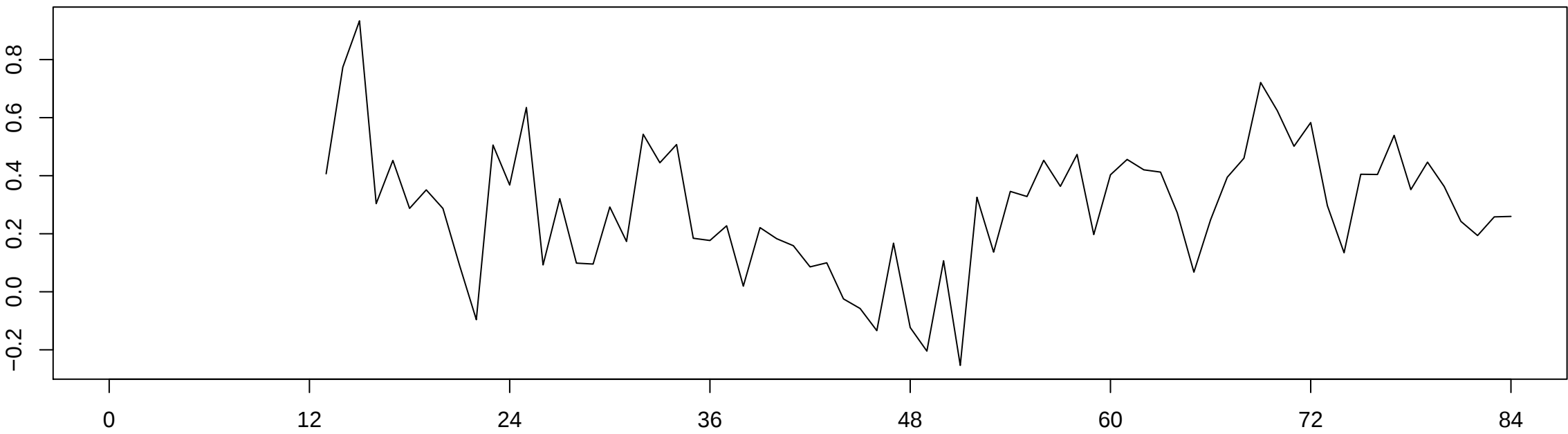
Differencing log(Z) at Lag 12
