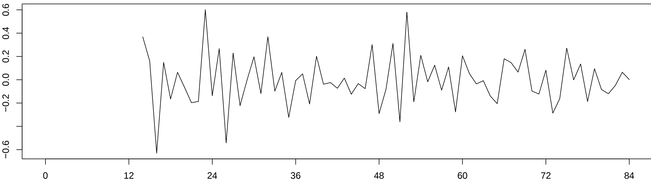
Differencing log(Z) at Lags 1 and 12
