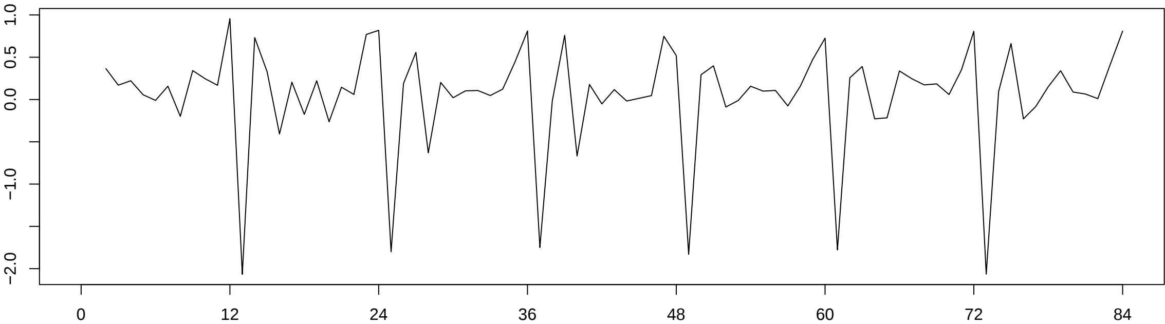
Differencing log(Z) at Lag 1
