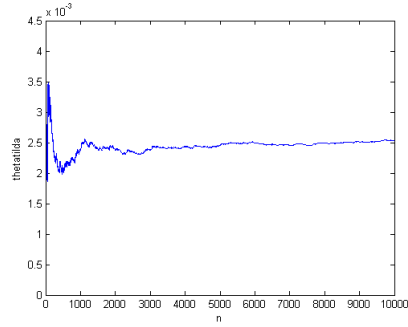
Figure 4.2: Convergence of Tilted Density for a=6 \lambda = 1
