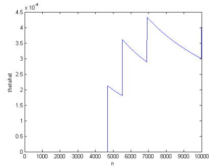
Figure 4.9: Convergence of Classical MC for a=8 and \lambda = 1
