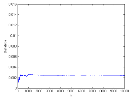
Figure 4.8: Convergence of Tilted Density for a=6 \lambda = 1
