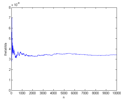
Figure 4.10: Convergence of Tilted Density for a=8 \lambda = 1
