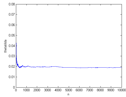
Figure 4.6: Convergence of Tilted Density for a=4 \lambda = 1
