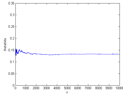
Figure 4.4: Convergence of Tilted Density for a=2 \lambda = 1
