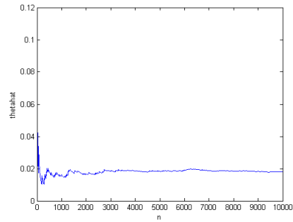
Figure 4.5: Convergence of Classical MC for a=4 and \lambda = 1
